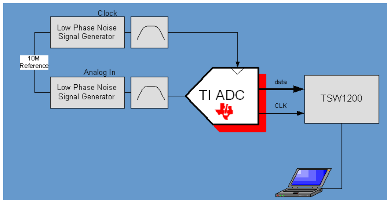
Figure 7. Test Setup Block Diagram
