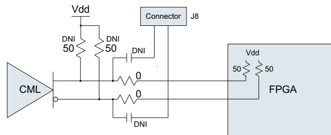
Figure 5. CML Termination Options
